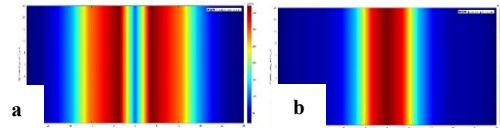
Figure 13. 35kV Ochistnye B line magnetic (a) and electric (b) field distribution map
